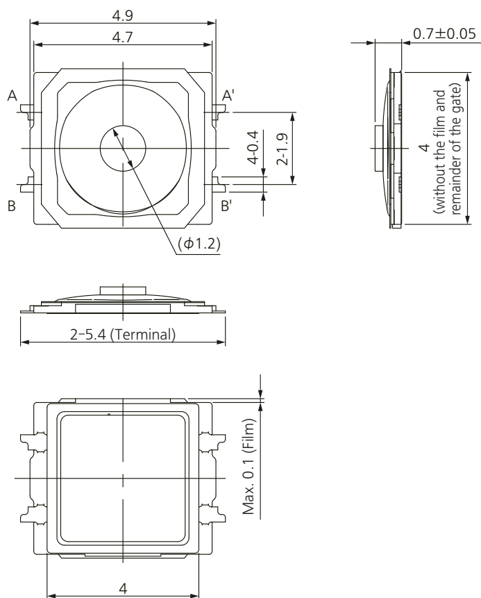
External dimensions
