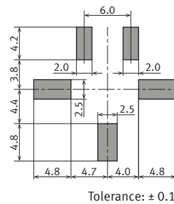
Recommendable mounting pad ( TOP VIEW )
