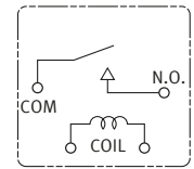
Schematic ( BOTTOM VIEW ) 1 Form A
