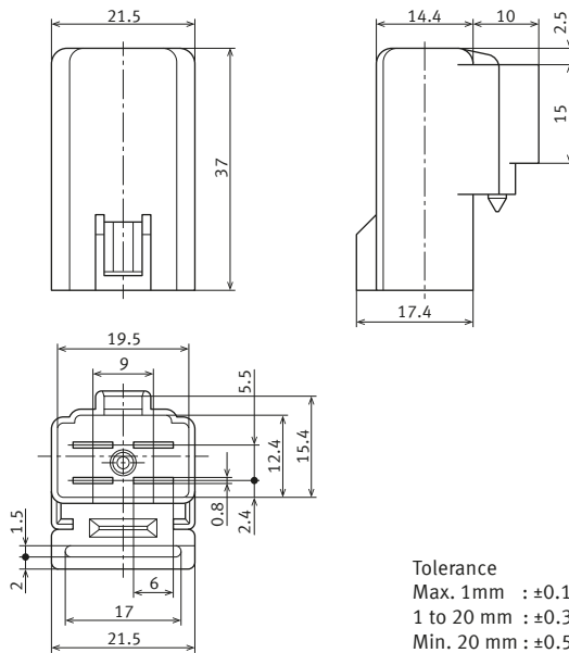
External dimensions
