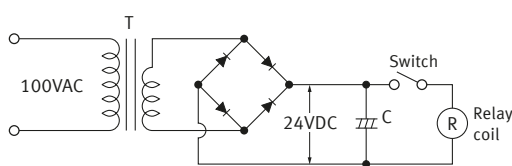
Fig. 2 Voltage fluctuation absorbing circuit using a condenser
