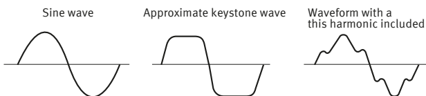
Fig. 1 Distortion in an AC stabilized power source
