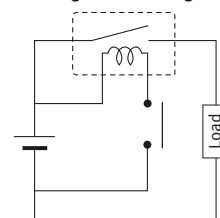
Fig. 4 Applied voltage and voltage drop of the coil
