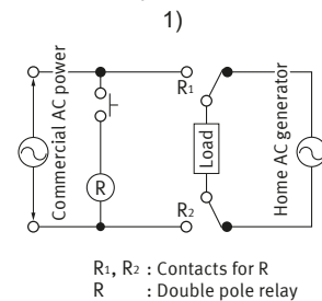
Fig. 16 Bad example of Form A and B use
