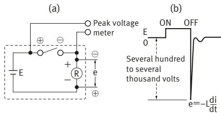
Fig. 13 Example of counter emf and actual measurement
