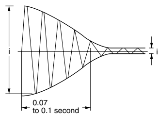
(5) Solenoid Load
