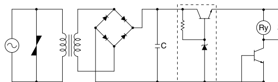
Fig. 1 Stabilized circuit (Example)
