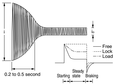
(4) Motor Load i/i_0 \approx 5 to 10 times
