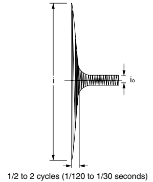
(7) Capacitive Load
