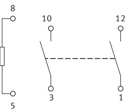
Schematic ( BOTTOM VIEW )
