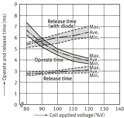
5-2. Operate and release time ( 1 Form A 1 Form B, 2 Form A )
