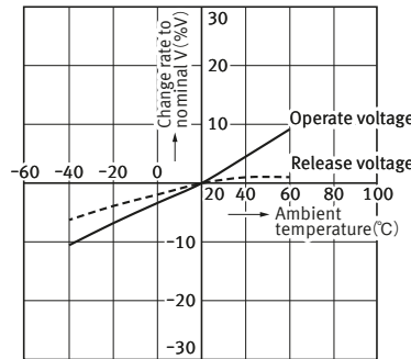
4-2. Ambient temperature characteristics ( 1 Form A 1 Form B, 2 Form A: Average )
