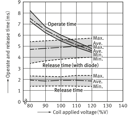
5-1. Operate and release time ( 1 Form A )
