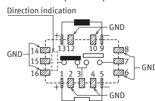
2 coil latching Standard contact ( Reset )
