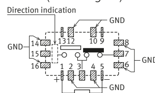
2 coil latching Standard contact ( Reset )
