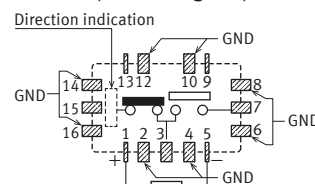
Reverse contact ( De-energize )
