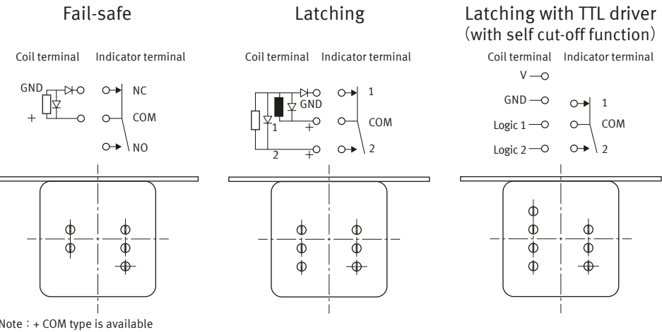
Solder terminal layout
