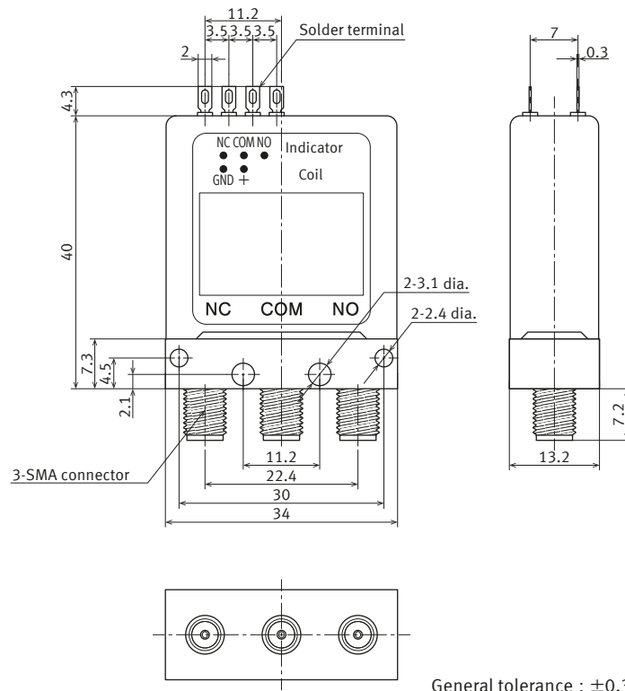
External dimensions
