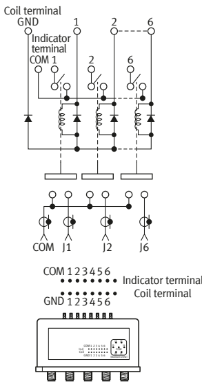
Solder terminal layout Fail-safe
