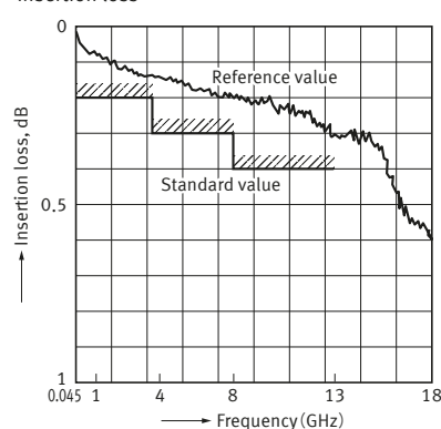
Insertion loss
