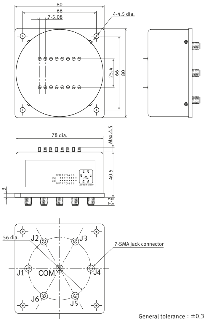
External dimensions
