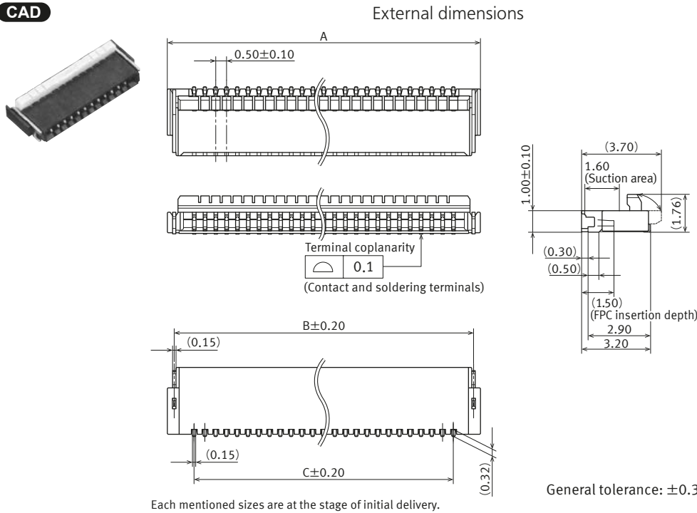
Dimension table
